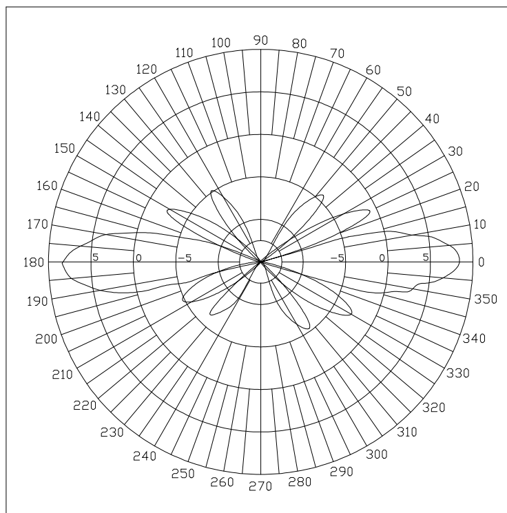
E-Plane Field Pattern
