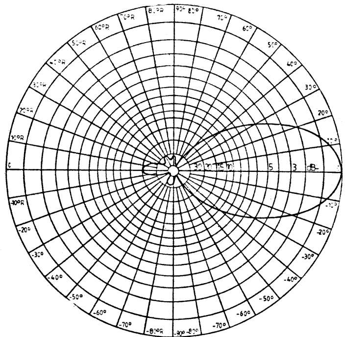
2m X-Quad
