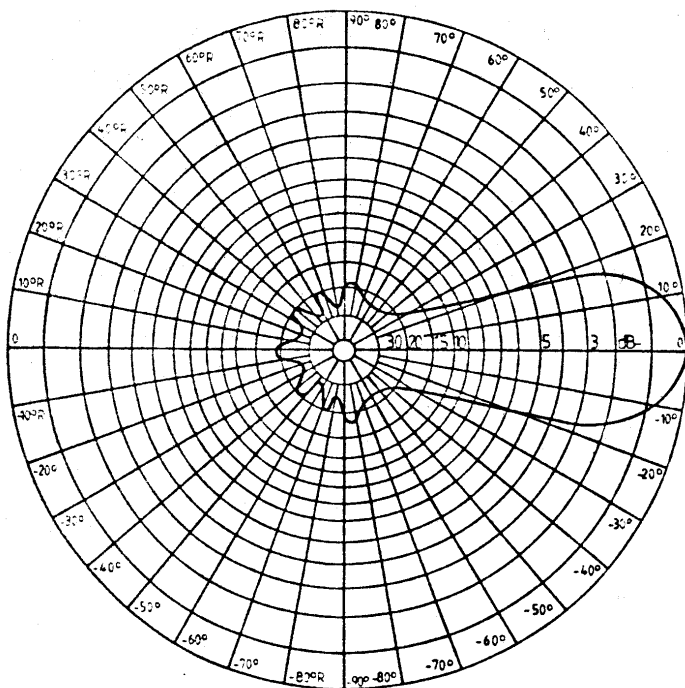
70cm X-Quad
