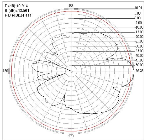
E plane
