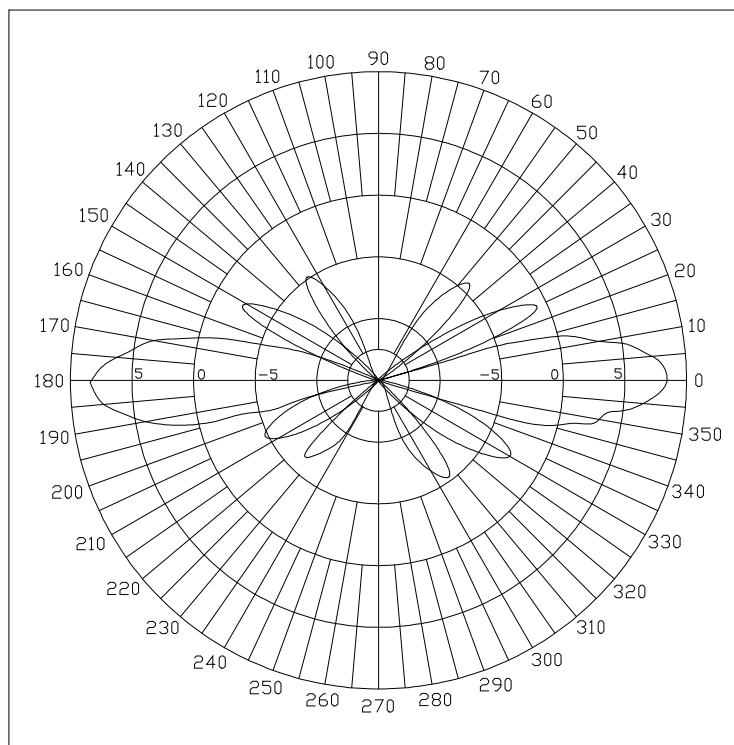
E-Plane Field Pattern
