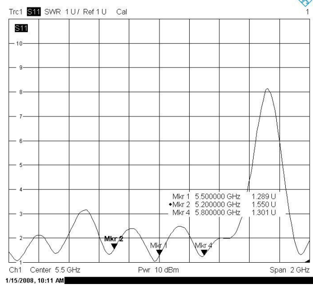
SWR
