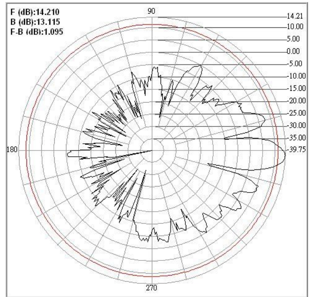
E plane
