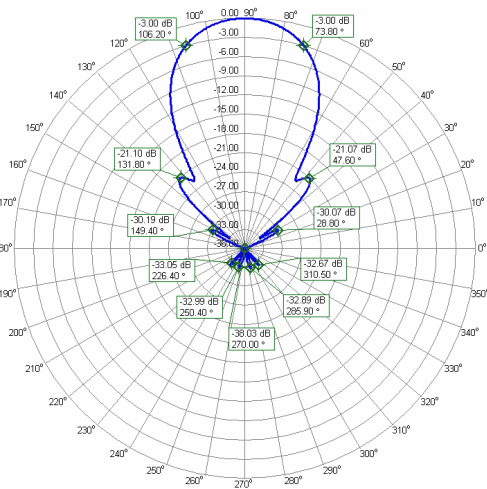
2 m Azimuth Radiation Pattern
