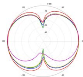
E-Ebene
