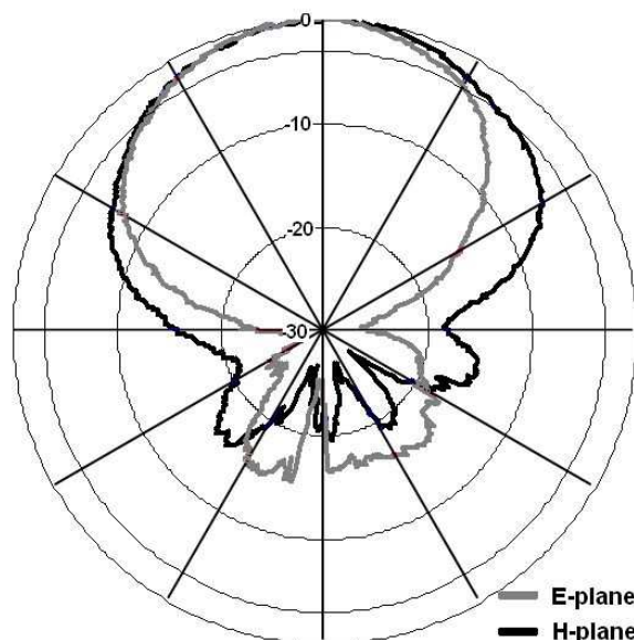
Radiation pattern:
