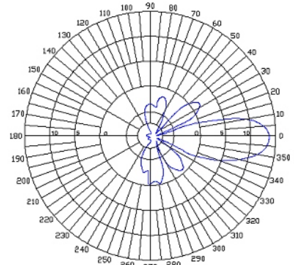
E-Plane Field Pattern
